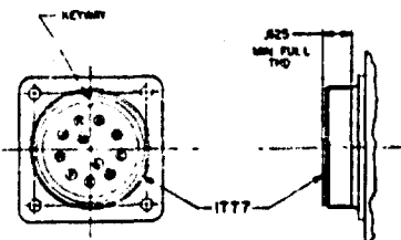
THIS CONNECTOR ACCOMMODATES ANY CONNECTOR THAT MATES WITH MS 300-20-33P TURBINE ENT TEMPERATURE THERMOCOUPLE SCHEMATIC OF PIN DESIGNATION SCALE: 2/1
